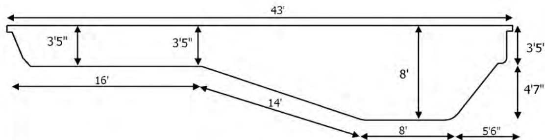
Depth Chart
