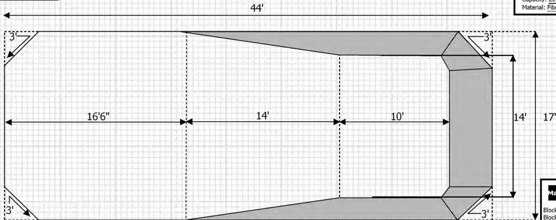
Outside Dimensions
