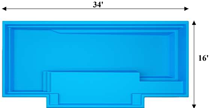
Outside Dimensions
